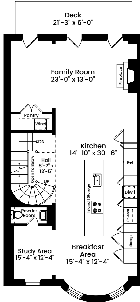
SECOND FLOOR CEILING HEIGHT 10'-0"
